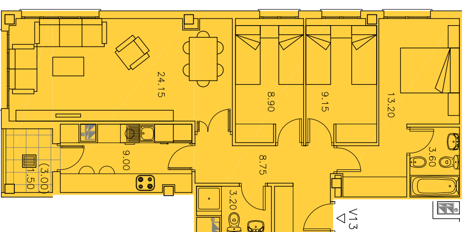
V13. SUP. ÚTIL TOTAL=81.45m2
